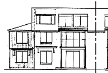
ELEVATION Private side (north)
