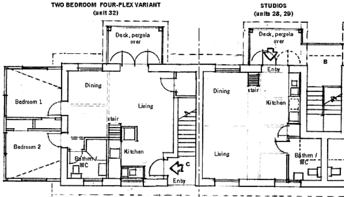
FLOOR PLANS 1:100 Upper level
