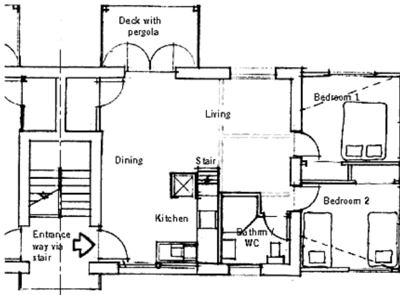
FLOOR PLAN 1:100 Main level
